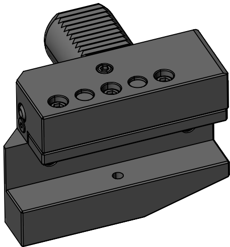
90 DEGREE VDI40 STATIC TOOL OUTPUT: 25mm SQR SHANK COOLANT: EXTERNAL
